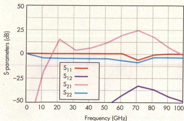
4. The LNA's measured S-parameters are: S_{11} < -9 dB; S_{21} (peak) = 25 dB; S_{12} < -35 dB; and S_{22} < -10 dB.
