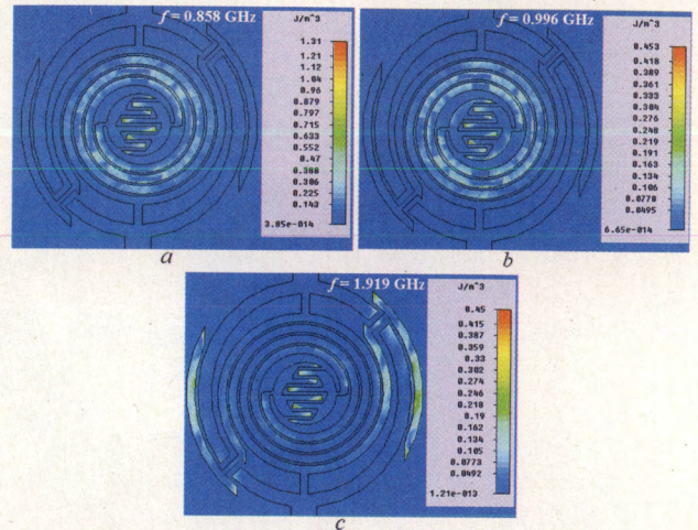
3. These plots show the measured electrical energy density of the BPF at 0.858 GHz (a), 0.996 GHz (b), and 1.919 GHz (c).
