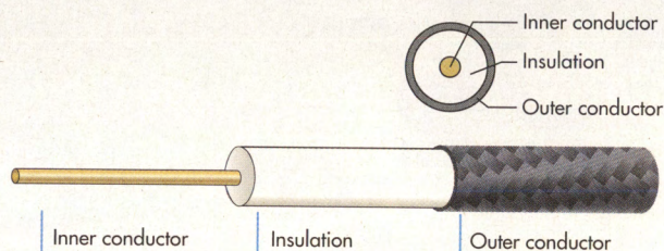
1. Two-conductor RF/microwave cables consist of inner and outer conductors separated by some form of dielectric material.
