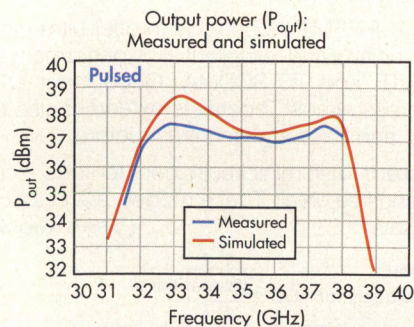
4. Close correlation between measured and simulated output-power performance indicates the quality of the circuit design and the simulation software.
