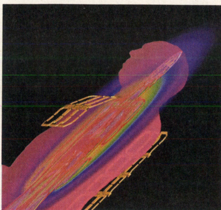
4. Some EM simulators may rely on multiple numerical solvers or combinations of solvers to achieve the most effective simulation results.
