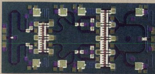
Figure 2. The operational two-stage MMIC amplifier, with a 3 mm input stage driving a 6 mm output stage, using on-chip matching and biasing.
