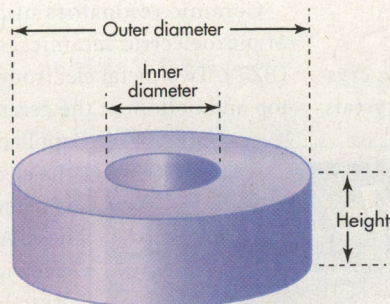
2. This illustration represents a typical disc-shaped dielectric resonator.
