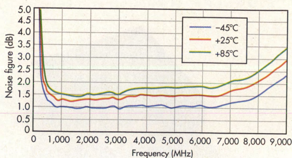
3. Noise figure is well controlled across the wide frequency range even when subjected to a wide range of operating temperatures.
