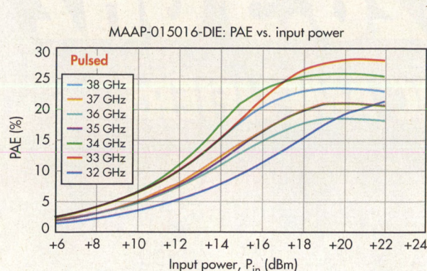
3. As the pulsed data shows, the GaAs MMIC PA achieves PAE between 18% and 27% across the full frequency range.
