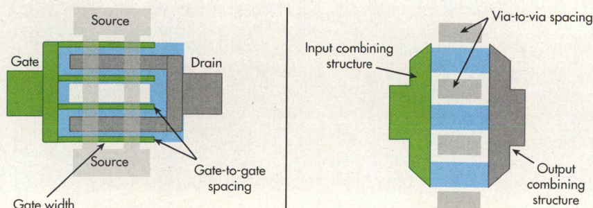
1. This layout shows the configuration of the Ka-band PA, including its multiple-cell combining structure.
