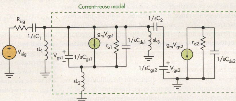
2. Shown is an equivalent-circuit small-signal model of the LNA (without the buffer).
