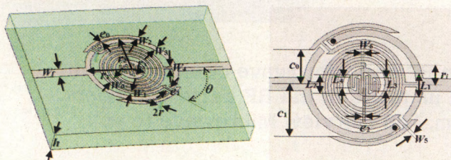
1. The compact BPF is shown in a three-dimensional (3D) view (left) and in a view from the top (right).
