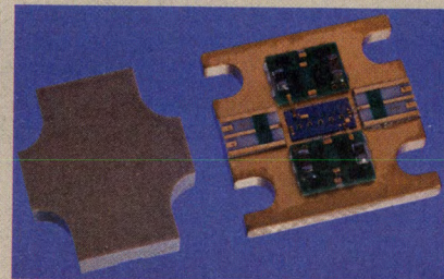
Figure 3. The CMPA0060002F was the first GaN MMIC in volume production, becoming available in 2008.
