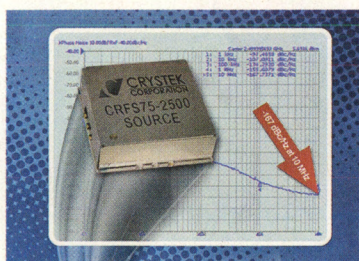
Model CRFS75-2500 is an SMT-packaged, PLL clock source with low-noise, fixed-sine-wave output of 2.5 GHz.
