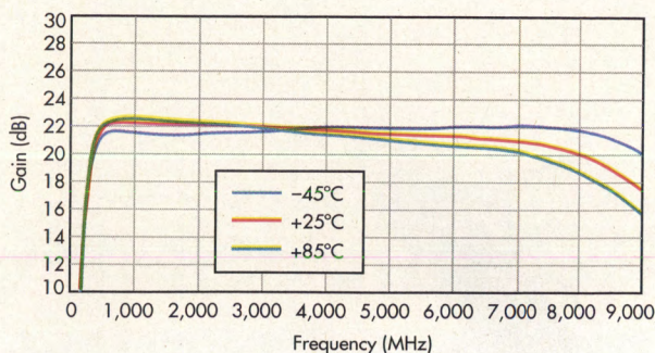
2. Amplifier gain remains steady across a wide operating-temperature range compared to room-temperature performance at +25°C.
