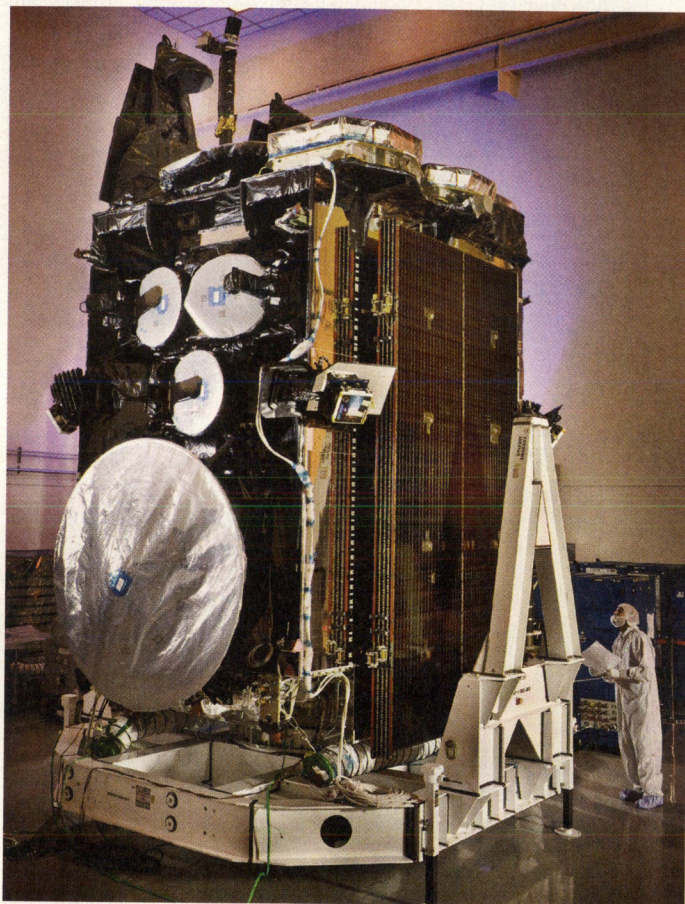
A technician inspects part of an AEHF satellite before it enters active service in support of U.S. military forces. (Image courtesy of Lockheed Martin)
