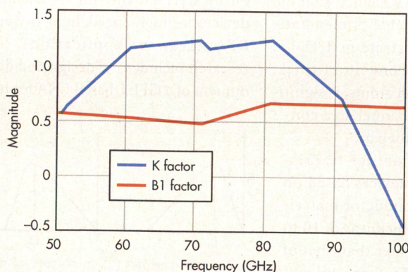
6. The LNA's K and B1 factors indicate excellent stability for the millimeter-wave circuit.
