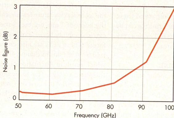
5. The LNA maintains noise figure of less than 0.6 dB across its operating bandwidth.
