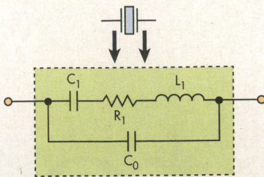
3. This electrical circuit represents a quartz crystal's electrical equivalent near a resonant frequency.
