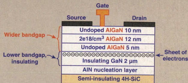
Figure 1. GaN/AlGaIn HEMT epilayer structure on a semi-insulating silicon carbide substrate.
