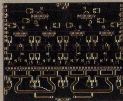
Figure 6. Cree's newest development is a high power Ku-Band MMIC providing 30 watts in the 13.5-14.75 GHz commercial satellite band.
