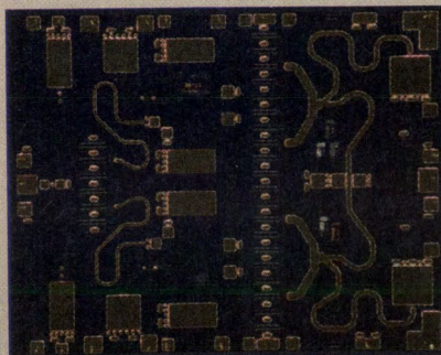
Figure 4. The first commercial MMICs from Cree were the CMPA0060005 and CMPA2560025 (shown here).
