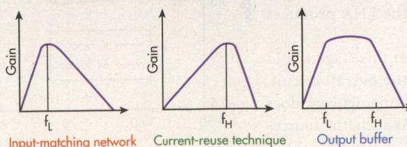
3. A stagger tuning technique helps to achieve the impedance matching needed for high wideband gain at millimeter-wave frequencies.
