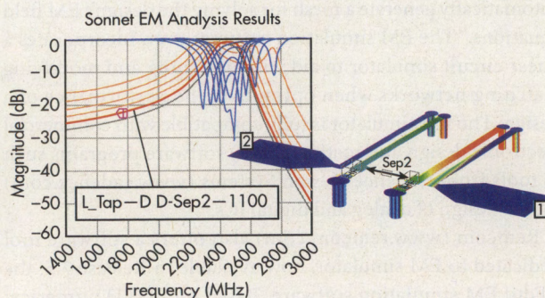
3. Planar 3D EM simulation software can model the EM field effects of transmission lines and interconnections at high frequencies, to help determine wideband performance. (Image courtesy of Sonnet Software)
