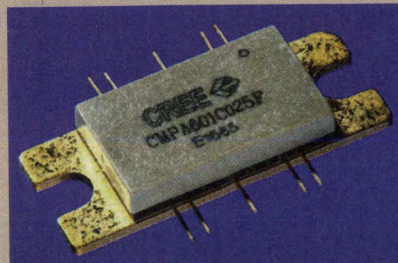
Figure 5. Wide bandwidth is the primary feature of the CMPA601C025F, which covers 6-12 GHz with 25 watts output power.
