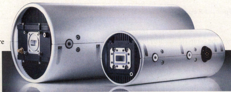
These SSPAs will soon be available for both Ku- and Ka-band, providing output power levels to 100 W and 50 W, respectively. (Courtesy of Mission Microwave Technologies)
