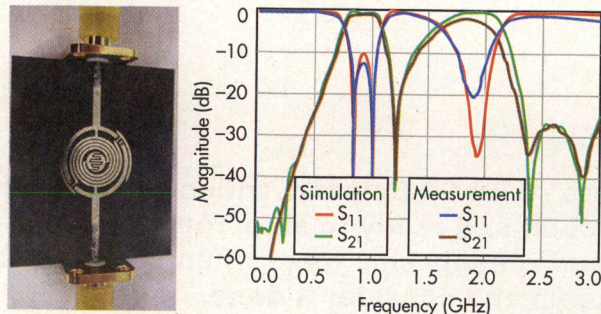
2. The fabricated BPF (left) achieved a close match between computer-simulated performance and actual measured performance (right).
